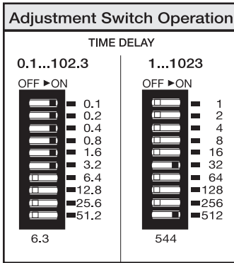
Add the value of switches in the ON position for the total time delay.
